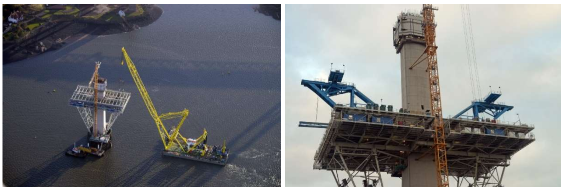
Figure 8 – Taklift 6 installed falsework, tower segments and erection gantries.
